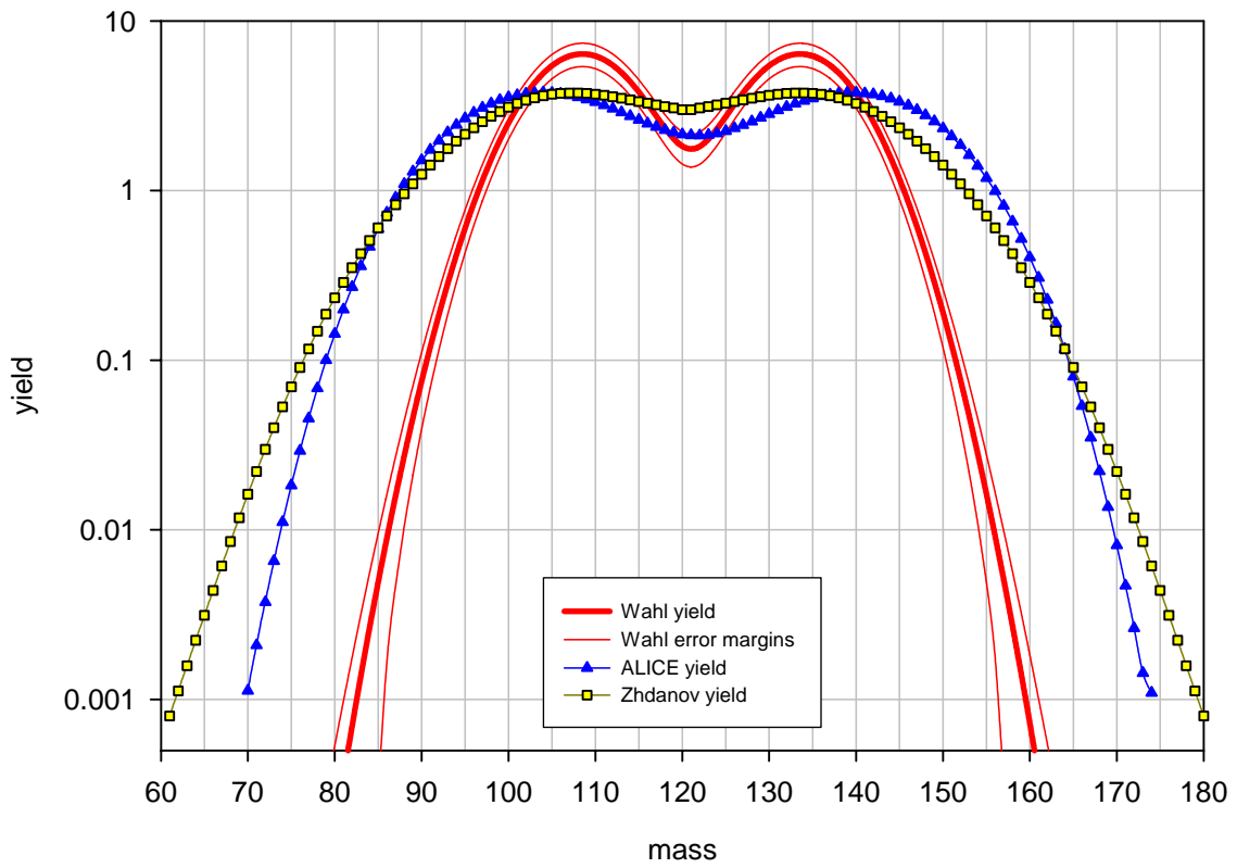
Benchmark B: ^{244}\text{Cm} at 50 MeV, pre-neutron emission mass distribution
